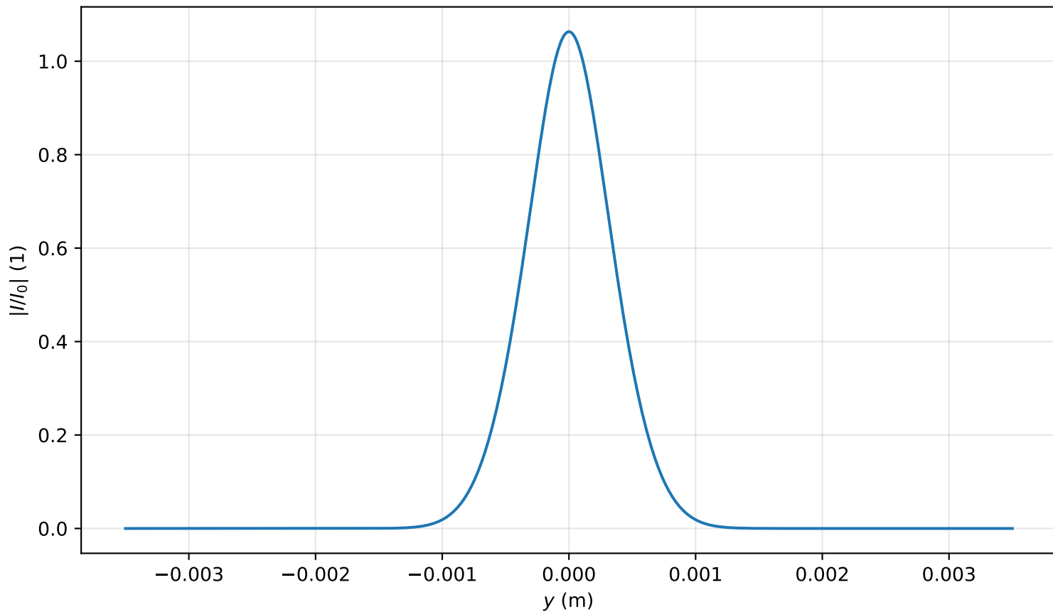
Intensity profile I(x=0, y, z=0.398)/I_0 , P_{in}=0.7P_{cr} , artificial time
